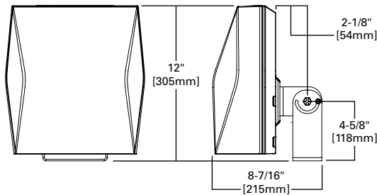
Trunnion Mount Detail
