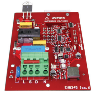
Universal Dimming Card
