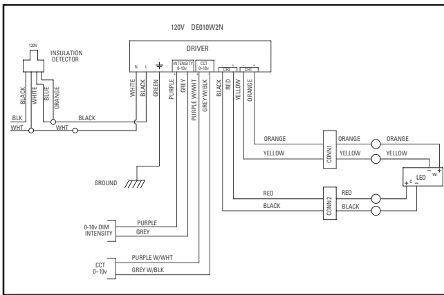
120V DE010W2N
