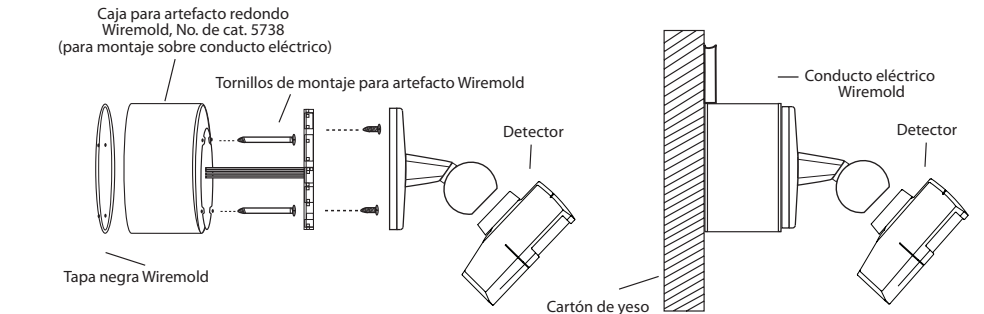
Occupancy Sensor Mounted to Round Fixture with Raceway
