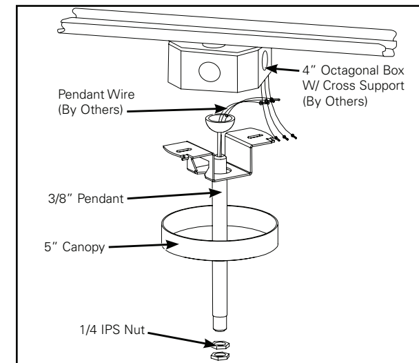
Figure 3. Power
