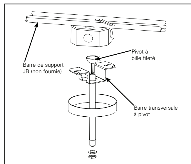
Figure 2. Sans alimentation
