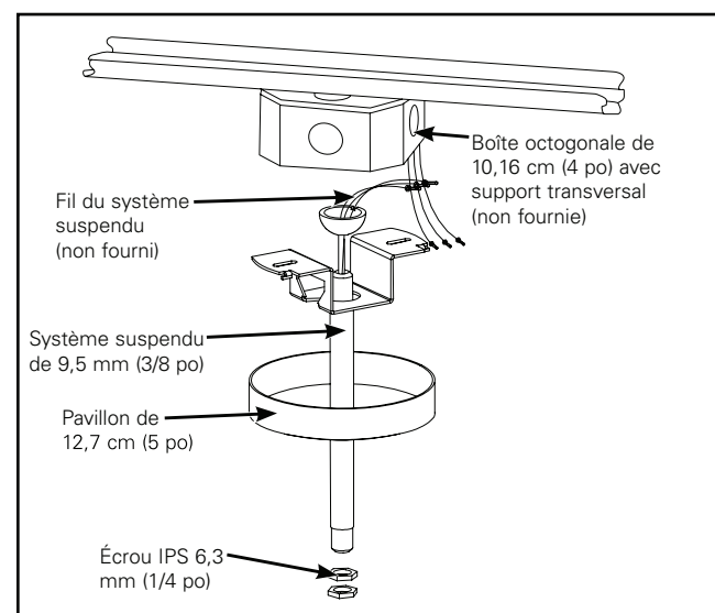
Figure 1. Alimentation
