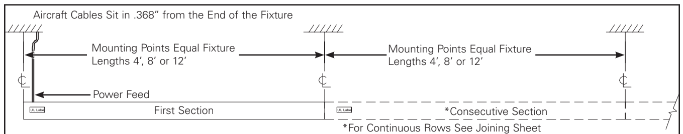
Figure 6. Mounts Locations
