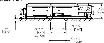
FLANGED TRIM
