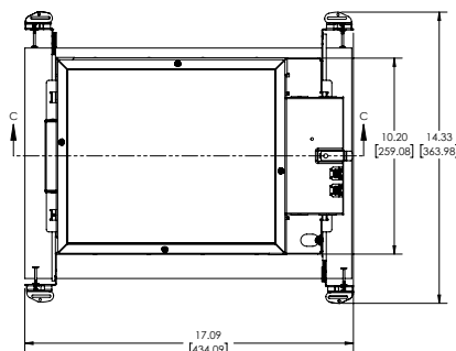
FLANGED TRIM
