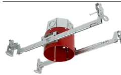
JB4FR2 4" NC JBox for Fire Rated Ceilings 4" diameter x 5-1/2" (102mm x 140mm)
