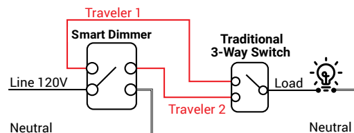
3-WAY APPLICATIONS (1) PURE SMART™ Wi-Fi® DIMMER SWW-DIM-WH (1) TRADITIONAL 3-WAY SWITCH
