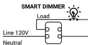
SINGLE-POLE APPLICATIONS (1) PURE SMART™ Wi-Fi® DIMMER SWW-DIM-WH
