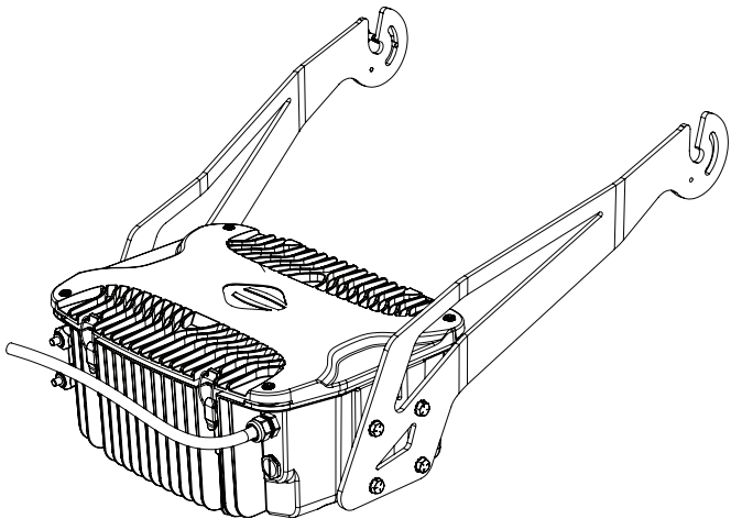
5b Closed Driver Box in Local Yoke Mount Configuration
