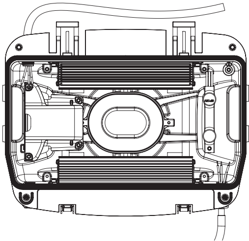
5b Closed Driver Box in Local Yoke Mount Configuration
