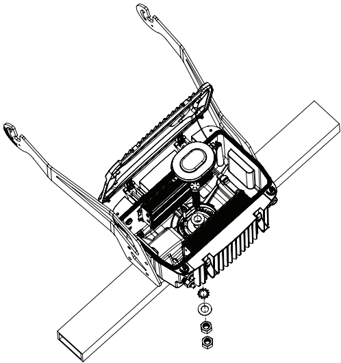
9 Local Yoke Mount
