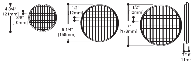
L275, L277, L279 Cube Louver
