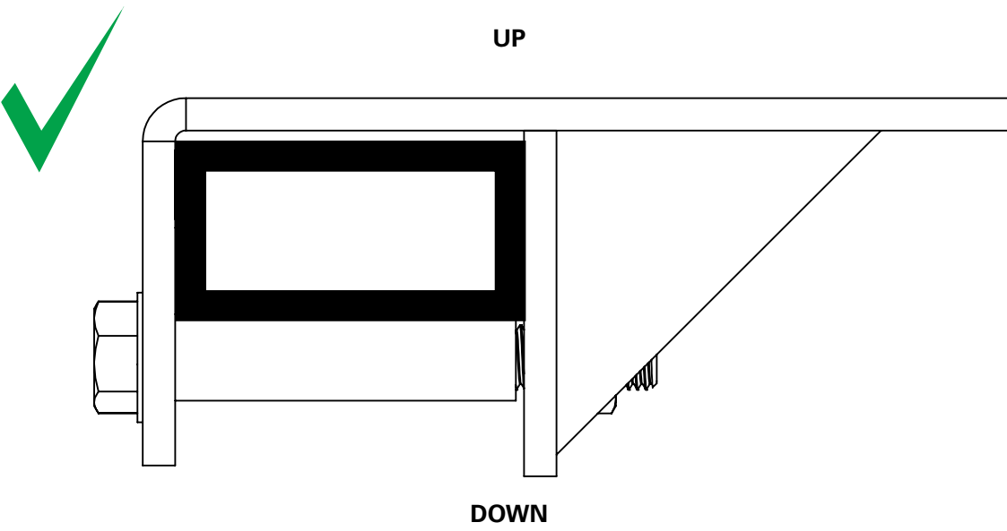
DB4a Correct Installation
