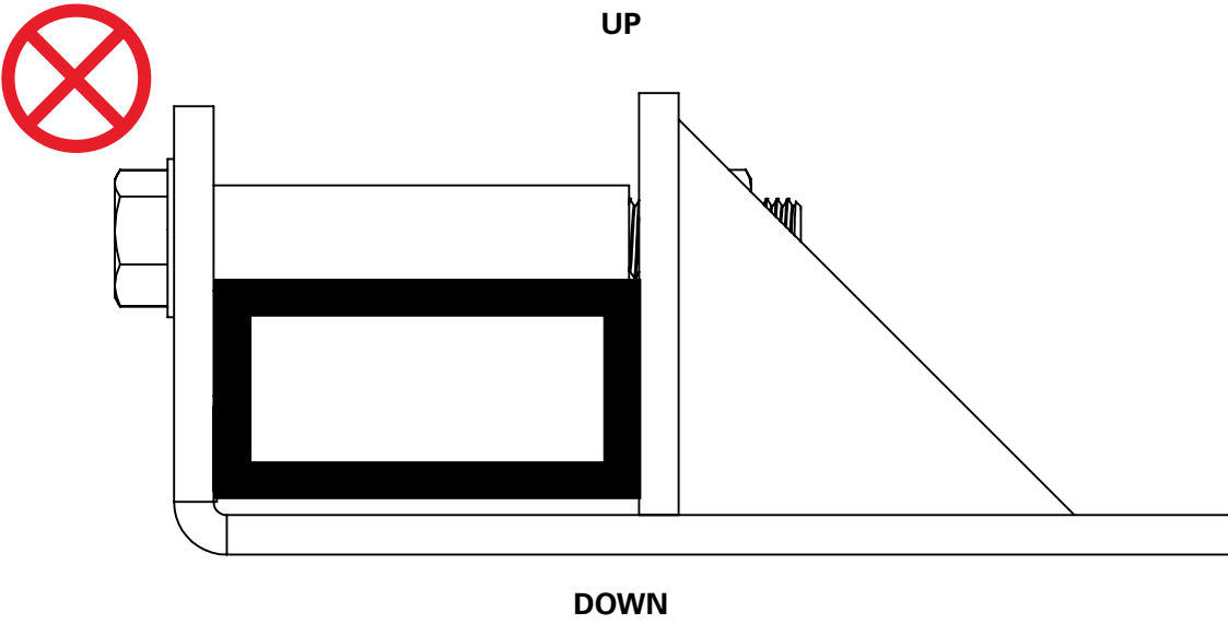
DB4b Incorrect Installation
